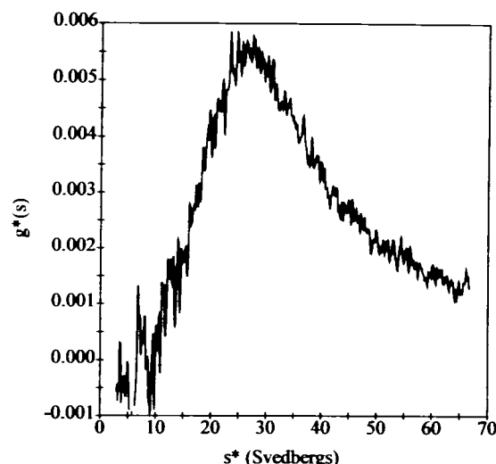
FIGURE 5 Apparent sedimentation coefficient distribution ( g^*(s) ) as a function of sedimentation coefficient. The data from Fig. 4 were fit using "dcdt" from Stafford (1992a,b) over the time range 38–63 min with \Delta t = 15 min. g^*(s) , exhibited a broad maximum near s = 27 S and a full-width-half-maximum over the range 17–42 S. The analysis is uncorrected for diffusion.
