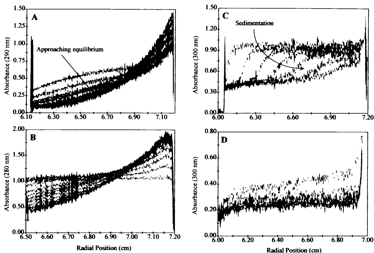
FIGURE 1 Sedimentation analyses of A \beta in different solvents. (A) Sedimentation equilibrium analysis of A \beta 40 dissolved in DMSO at 3 mg/ml (690 \mu M), centrifuged at 60,000 rpm ( 250,000 \times g ) for 64 h (6-h intervals between scans) at 23°C. The spike at about 6.15 cm is the solution meniscus. To calculate the molecular weight for a sedimenting component, independent determination of the partial specific volume ( \bar{v} ) of the protein is required. A search of Chemical Abstracts (Chemical Abstract Services, American Chemical Society, Columbus, OH) did not reveal any earlier reports of determinations for proteins in DMSO. When we used the monomeric molecular weight observed by ESI-MS (4325 Da) for A \beta 40 we calculated \bar{v} = 0.859 for monomer. To obtain dimer (8650 Da) required \bar{v} = 0.884 . (B) Sedimentation equilibrium analysis of A \beta 42 dissolved in DMSO at 3 mg/ml (670 \mu M) under the same conditions as in (A) (at 4-h intervals). As with A \beta 40 we used the molecular weight from ESI-MS (4511 Da) to estimate that \bar{v} = 0.858 for A \beta 42 in DMSO. Dimeric A \beta 42 would require that \bar{v} = 0.883 . (C) Sedimentation velocity analysis of A \beta 40 freshly dissolved in 30% ACN/0.1% TFA at 3 mg/ml centrifuged at 30,000 rpm ( 65,000 \times g ) for 1 h (at 12-min intervals) at 23°C. (D) Sedimentation velocity analysis of A \beta 42 freshly dissolved in 30% ACN/0.1% TFA at 3 mg/ml centrifuged at 3000 rpm ( 650 \times g ) for 1 h (4-min intervals) at 23°C. The large amount of noise on the raw data could be attributed to oil deposits on the optical system of the XL-A ultracentrifuge. This noise limits our ability to estimate parameter uncertainties on the measurements, but does not perturb the trends in the results that we present.
