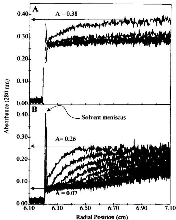
FIGURE 3 A \beta 40 (2 mg/ml, 450 \mu M) dissolved and aged in PBS (50 mM phosphate, 150 mM NaCl, pH 7.40), 23°C. Optical transients collected at 280 nm. (A) Rotor velocity of 3000 rpm ( 650 \times g ) presented at 6-min intervals showing the sedimentation of large aggregates. Sedimentation analysis of these aggregates gave a sedimentation coefficient of 50,000 S. (B) Rotor velocity of 30,000 rpm ( 65,000 \times g ) presented at 4-min intervals showing the sedimentation of smaller, “soluble” aggregates. Analysis yielded s \sim 30 S. From the indicated absorbance the relative contributions of large aggregates, soluble aggregates, and small species can be estimated.
